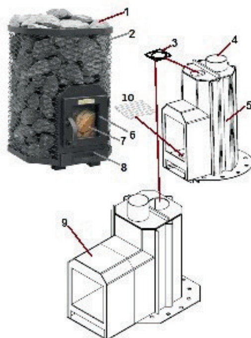
Figure 1. Heater components
